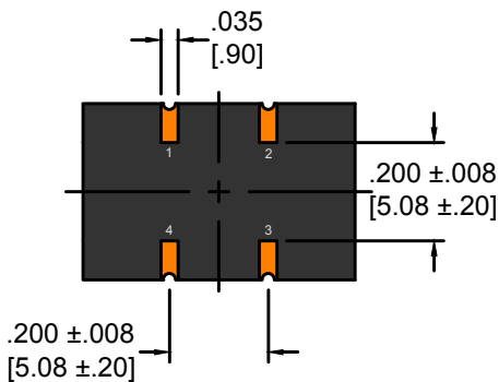
Recommended Pad Layout (Top View)
