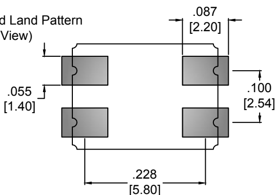
Recommended Land Pattern (Top View)
